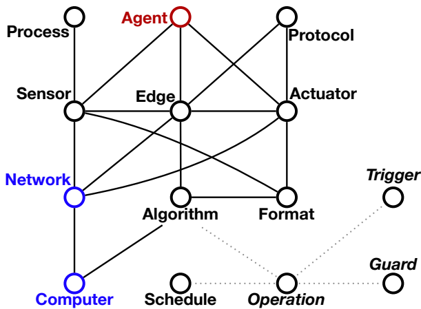
Figure 1. A graphical view of a CPS ontology. Nodes represent BWW [86] Things (in regular font) and Events (in italics), solid lines show Couplings, dotted gray lines denote other associations. Black labelled nodes are a part of the System, blue nodes may or may not be considered to be a part of the System (depending on whether the focus is on embedded systems or on pervasive computing), red nodes are traditionally viewed as a part of the Environment.
